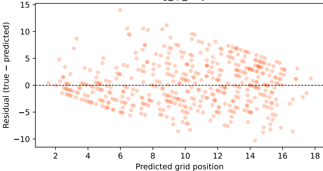
GradientBoosting_fp_only: Residual Plot
