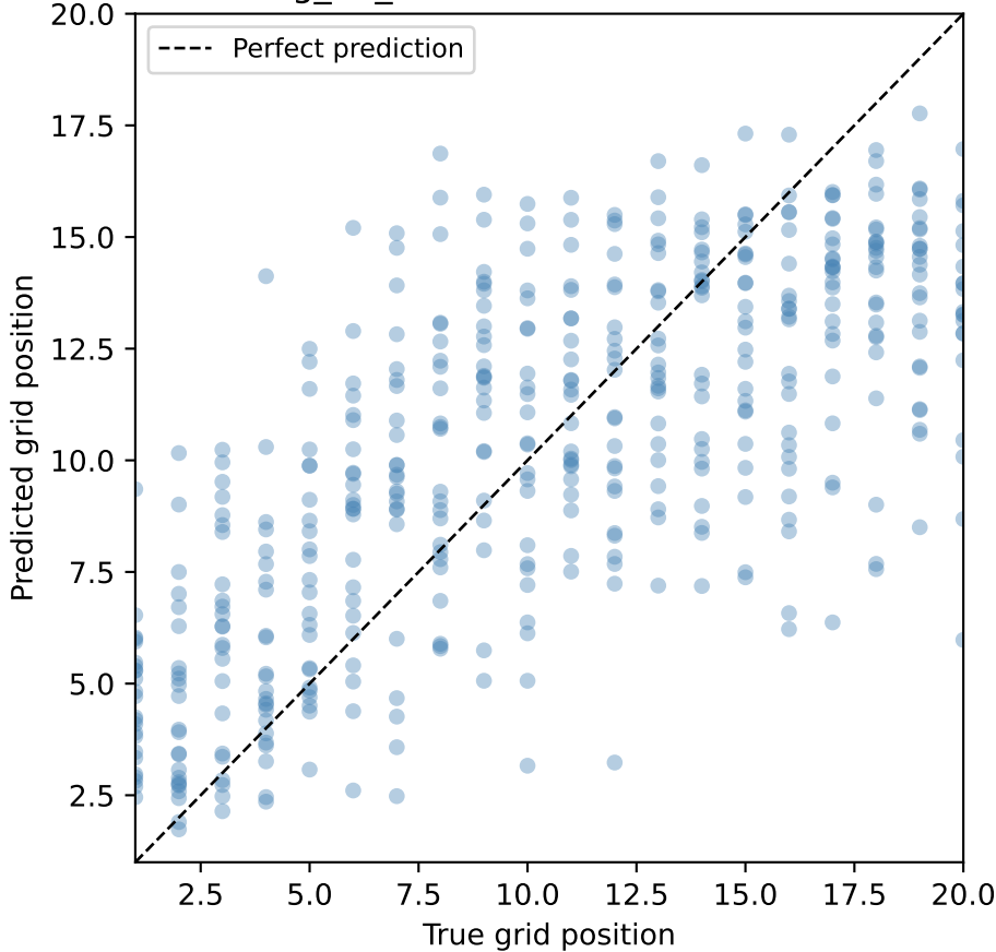
GradientBoosting_no_weather: Predicted vs True Grid Position
