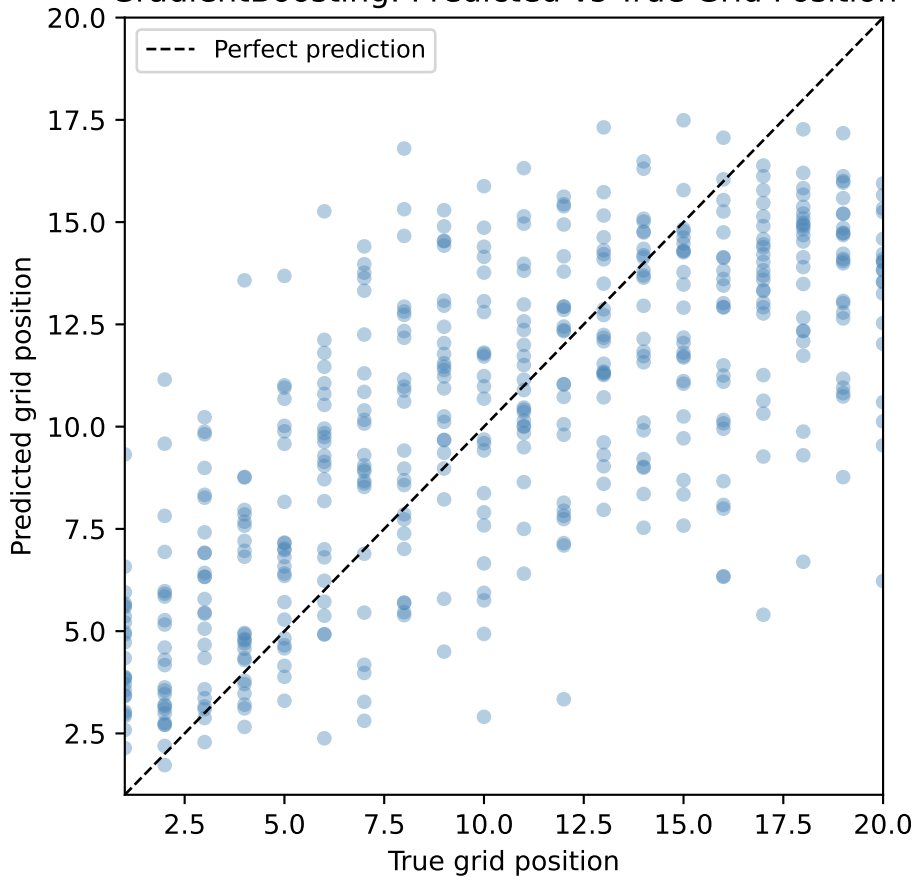
GradientBoosting: Predicted vs True Grid Position
