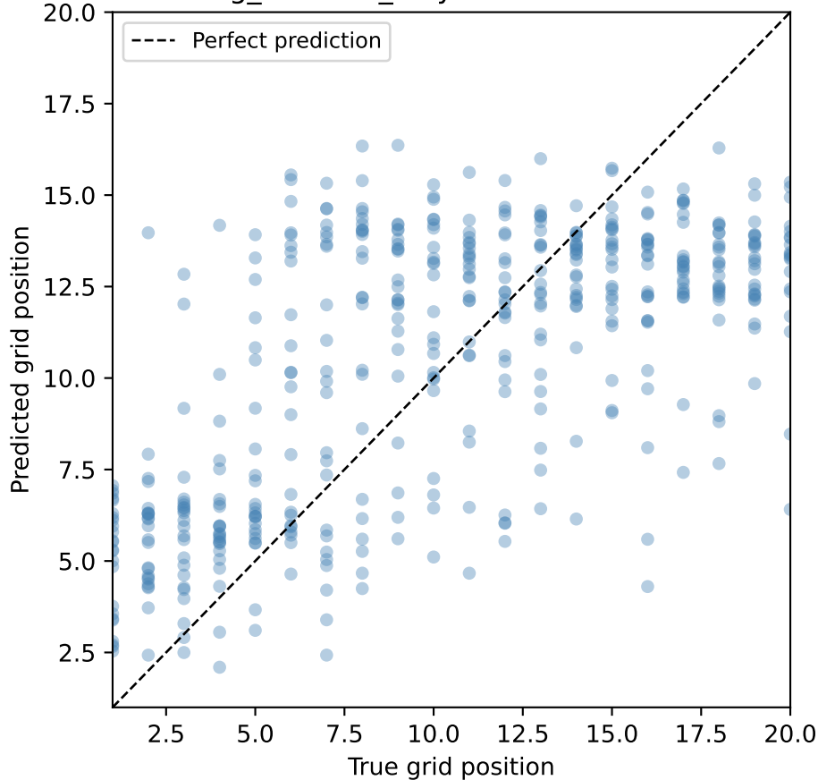
GradientBoosting_weather_only: Predicted vs True Grid Position
