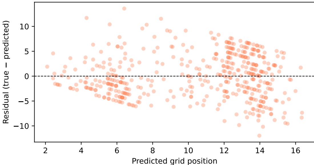
GradientBoosting_weather_only: Residual Plot
