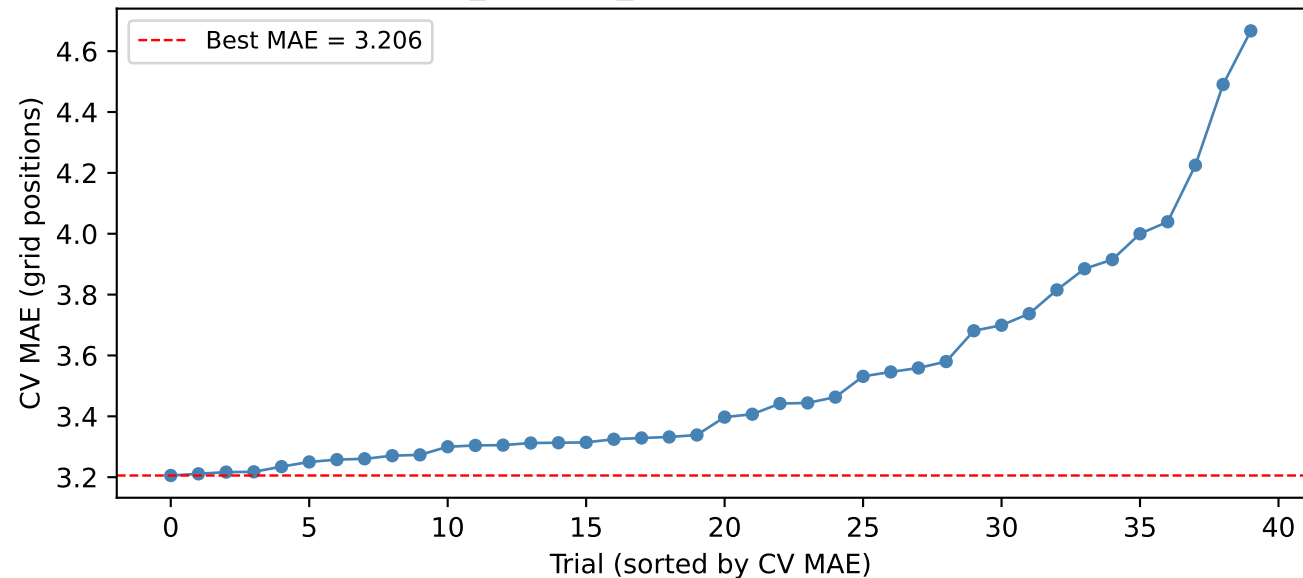
GradientBoosting_weather_only: Hyperparameter Search Results
