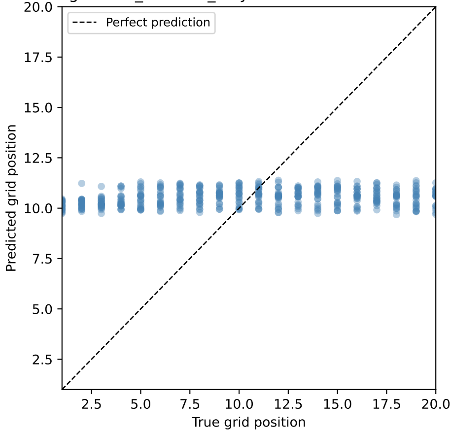
LinearRegression_weather_only: Predicted vs True Grid Position
