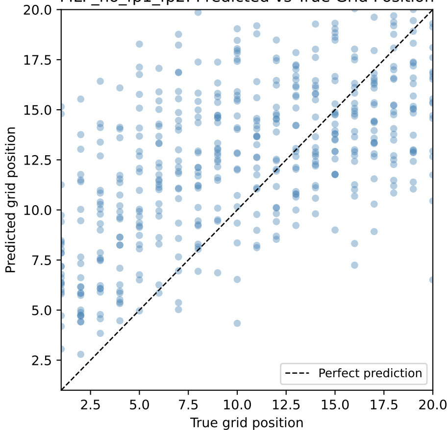
MLP_no_fp1_fp2: Predicted vs True Grid Position
