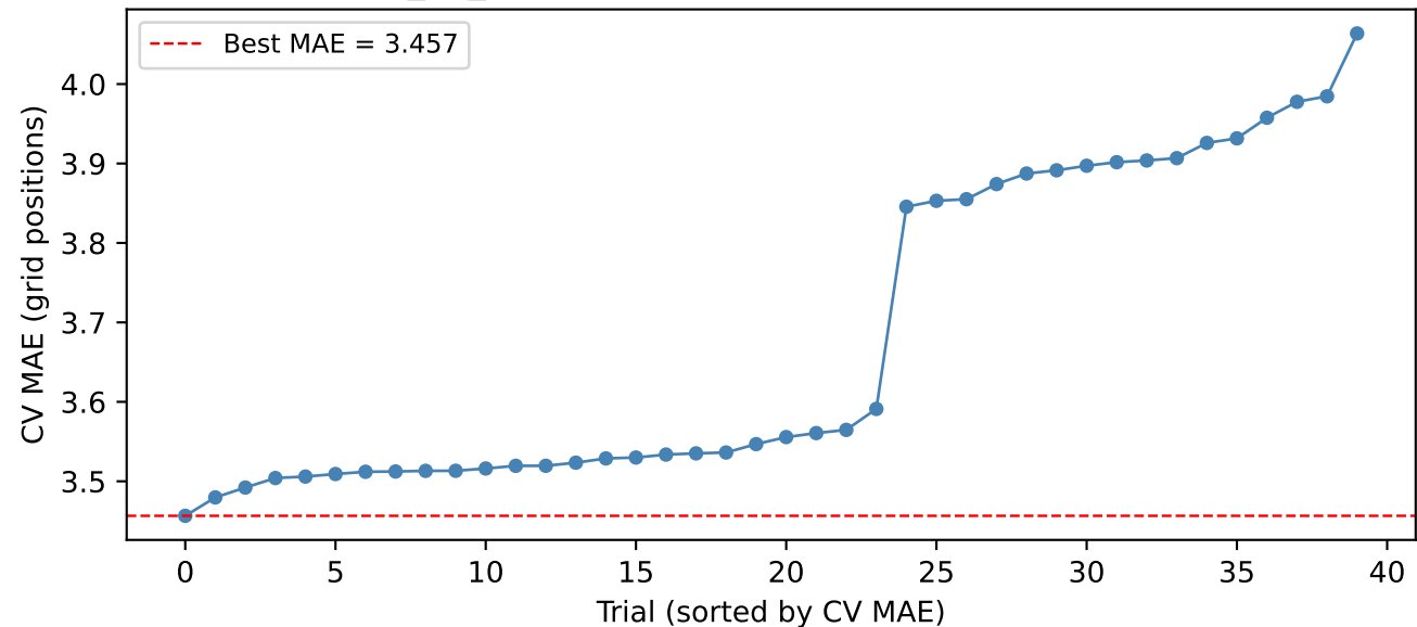
MLP_no_weather: Hyperparameter Search Results
