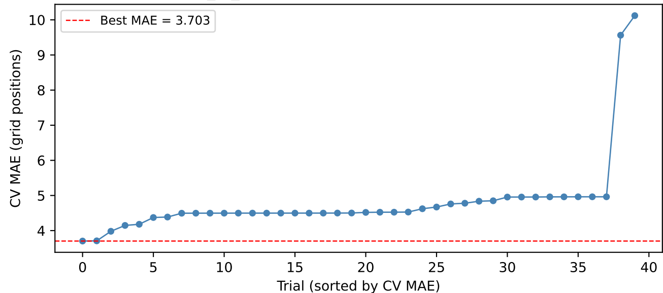
SVR_fp_only: Hyperparameter Search Results
