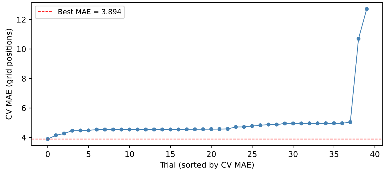
SVR_no_fp1: Hyperparameter Search Results
