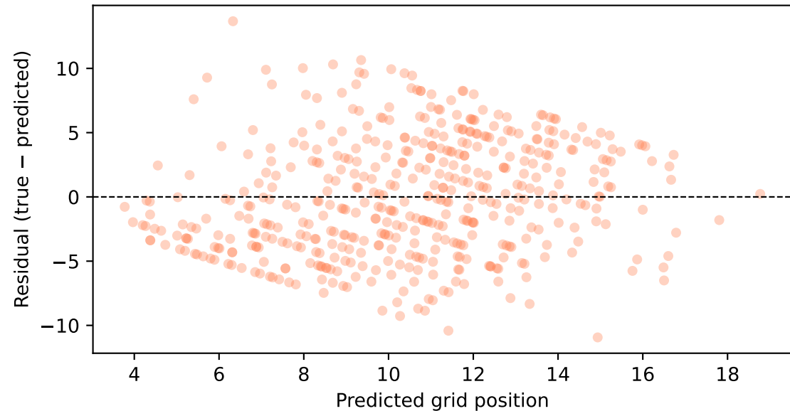
SVR_no_weather: Residual Plot
