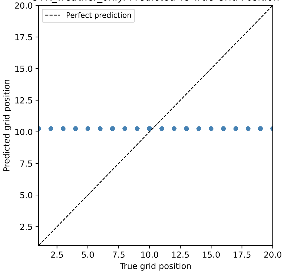
SVR_weather_only: Predicted vs True Grid Position
