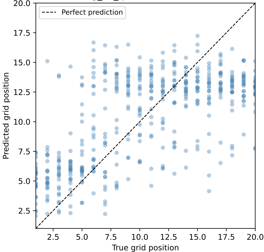
GradientBoosting_no_fp: Predicted vs True Grid Position
