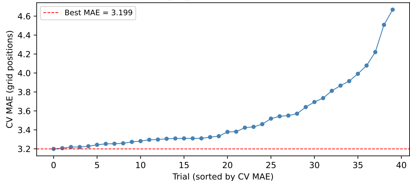
GradientBoosting_no_fp: Hyperparameter Search Results
