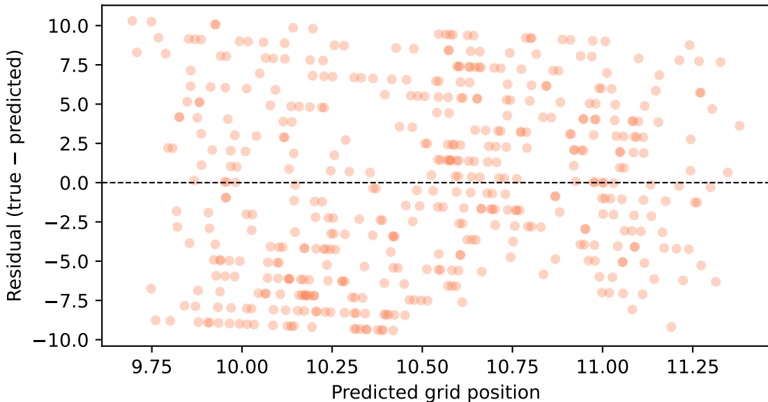
LinearRegression_no_fp: Residual Plot
