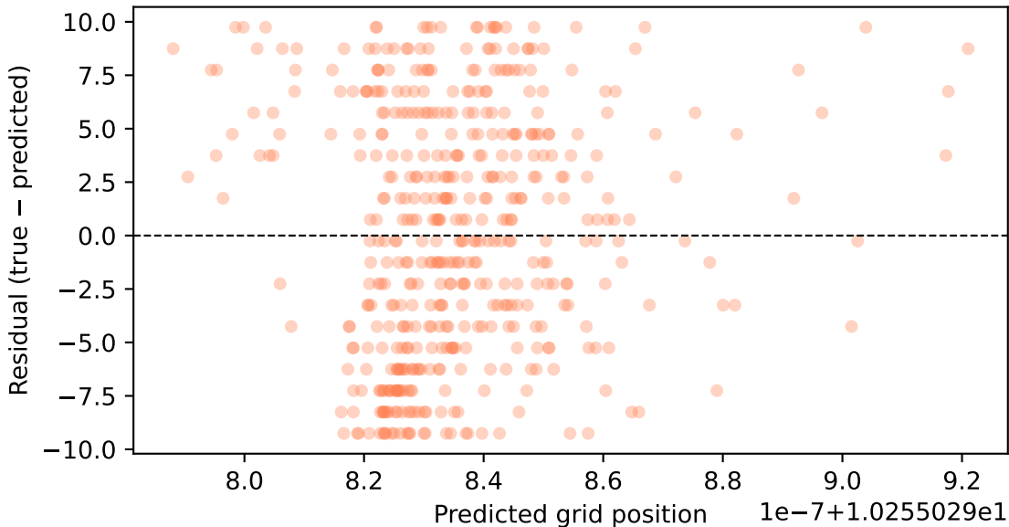
SVR_no_fp: Residual Plot
