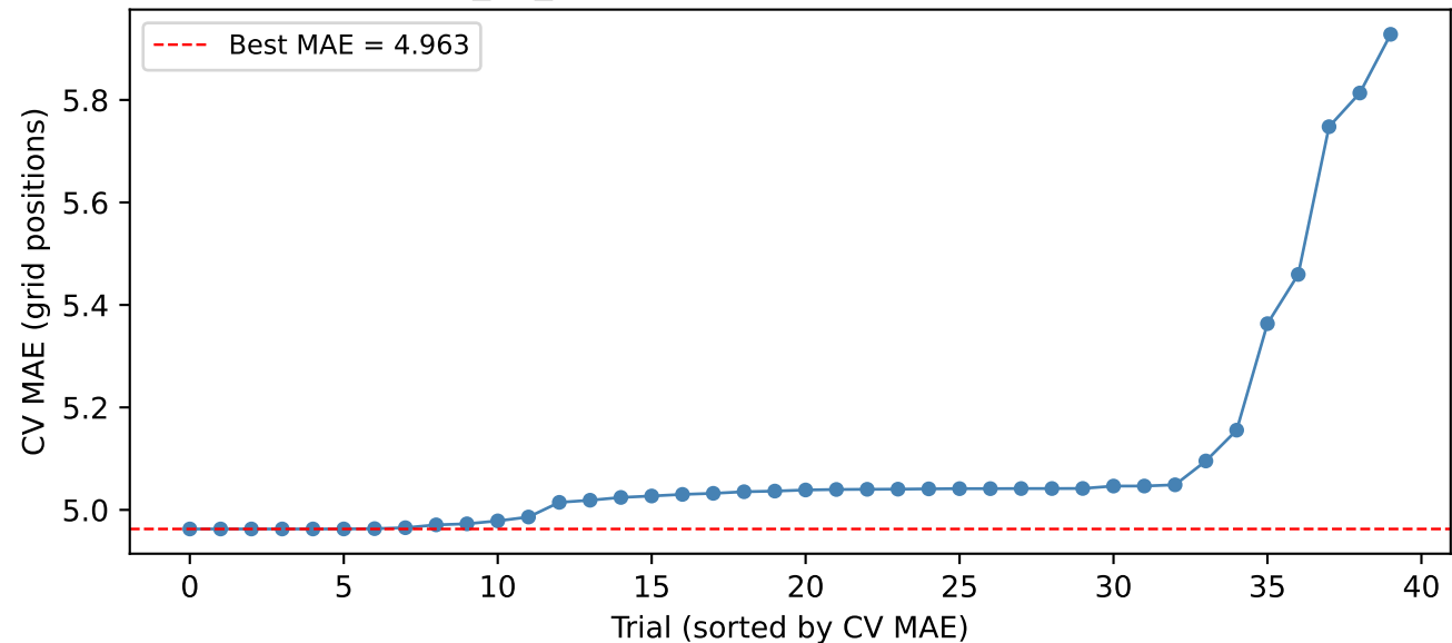
SVR_no_fp: Hyperparameter Search Results
