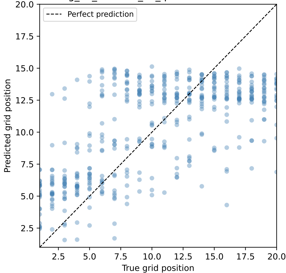
GradientBoosting_no_weather_no_fp: Predicted vs True Grid Position
