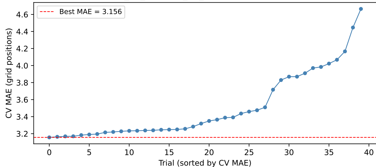
GradientBoosting_no_weather_no_fp: Hyperparameter Search Results
