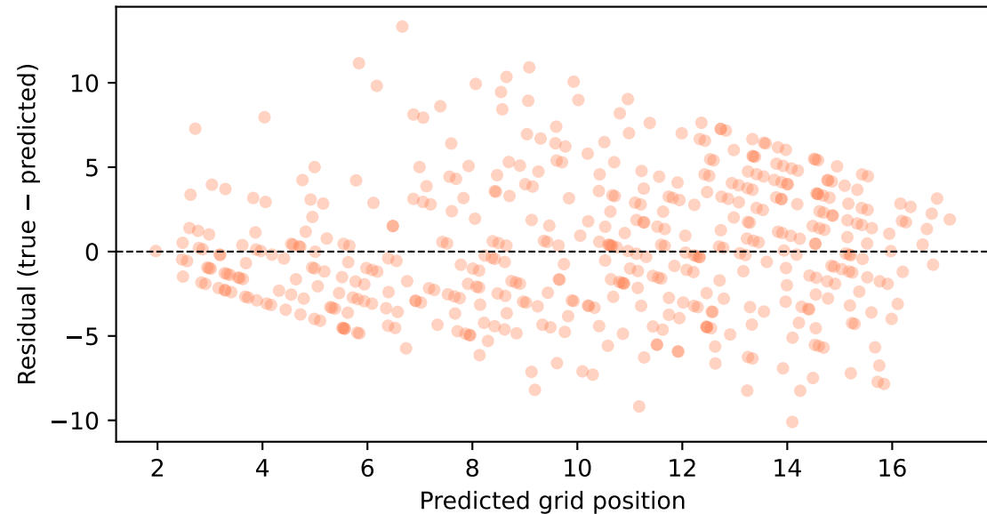
GradientBoosting_no_weather: Residual Plot
