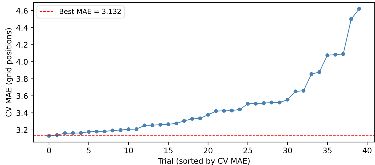
GradientBoosting_no_weather: Hyperparameter Search Results
