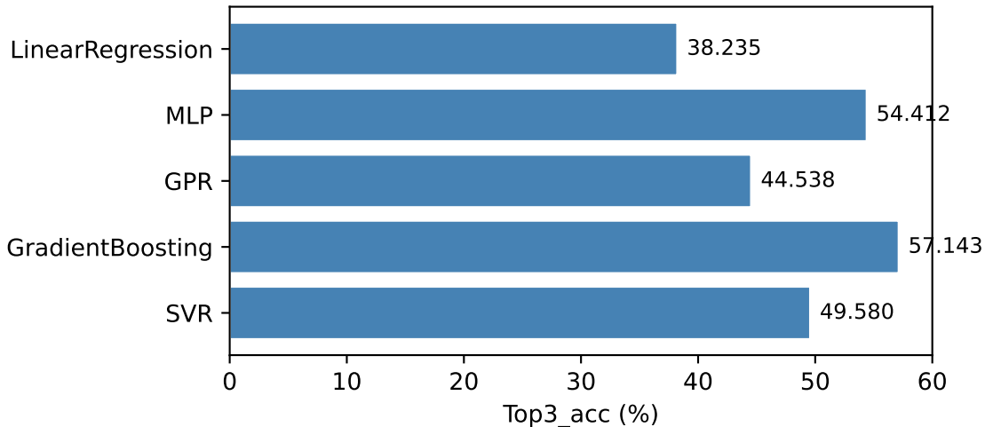
Model comparison — Top3_acc (%)
