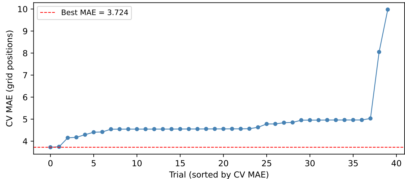
SVR: Hyperparameter Search Results
