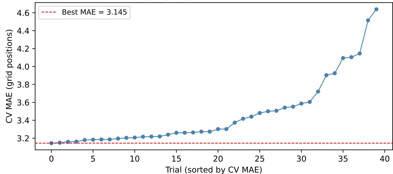
GradientBoosting_no_fp1_fp2: Hyperparameter Search Results
