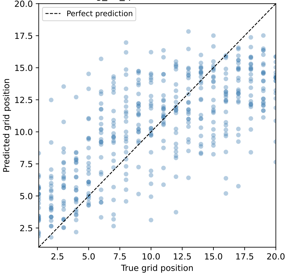
GradientBoosting_no_fp1: Predicted vs True Grid Position
