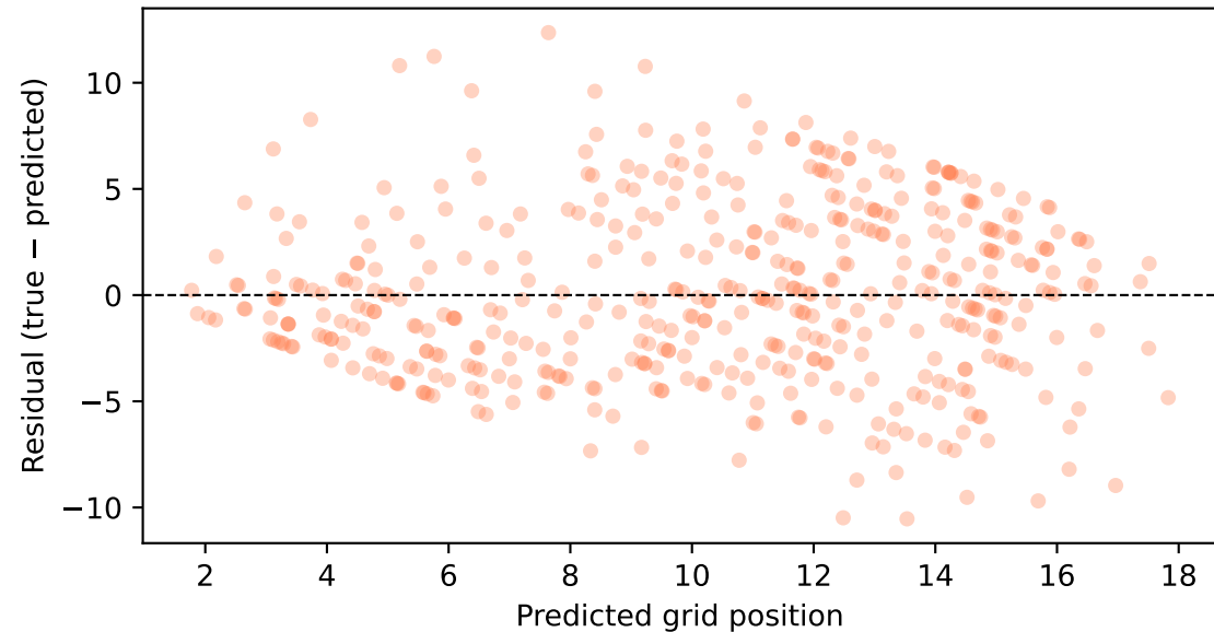
GradientBoosting_no_fp1: Residual Plot
