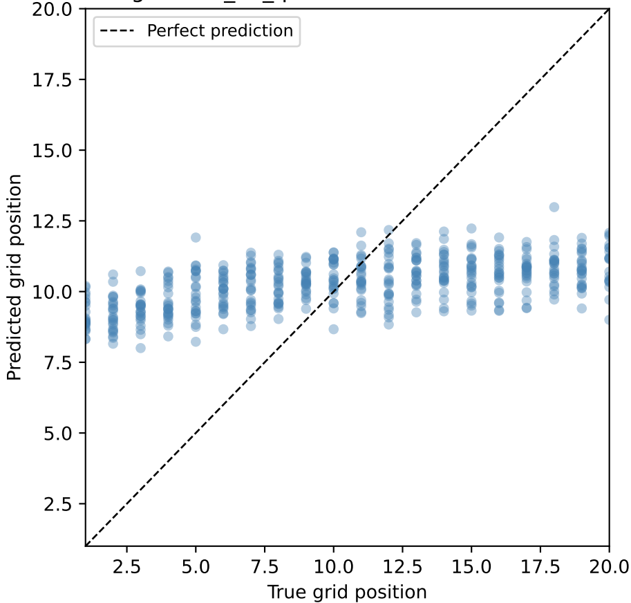
LinearRegression_no_fp1: Predicted vs True Grid Position
