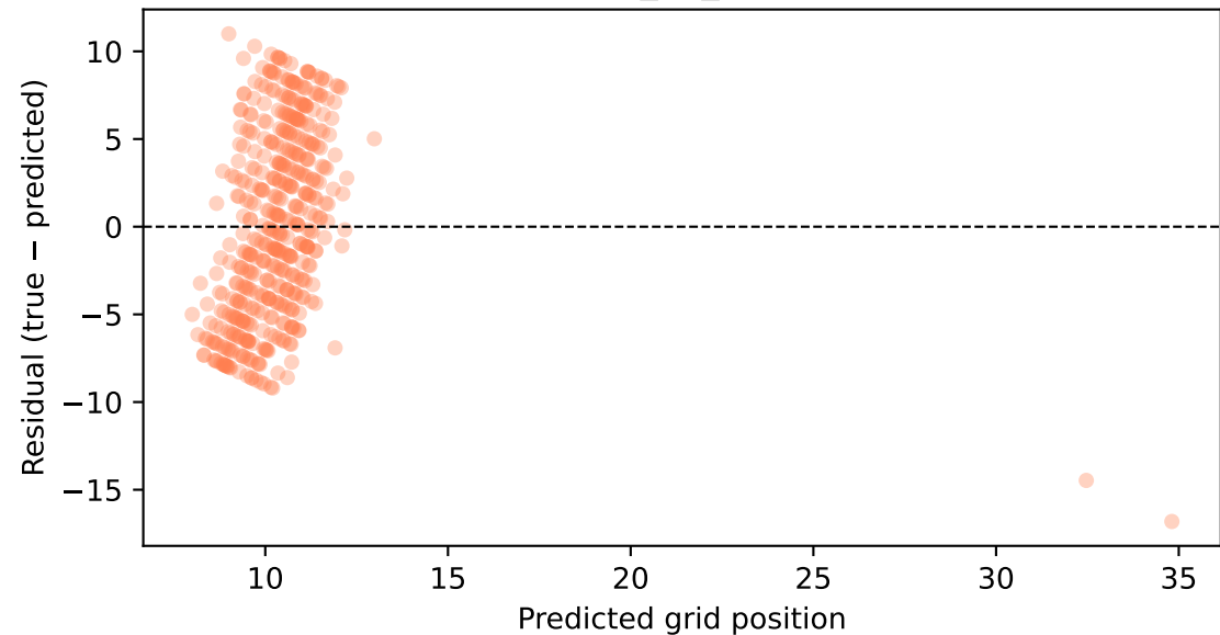
LinearRegression_no_fp1: Residual Plot
