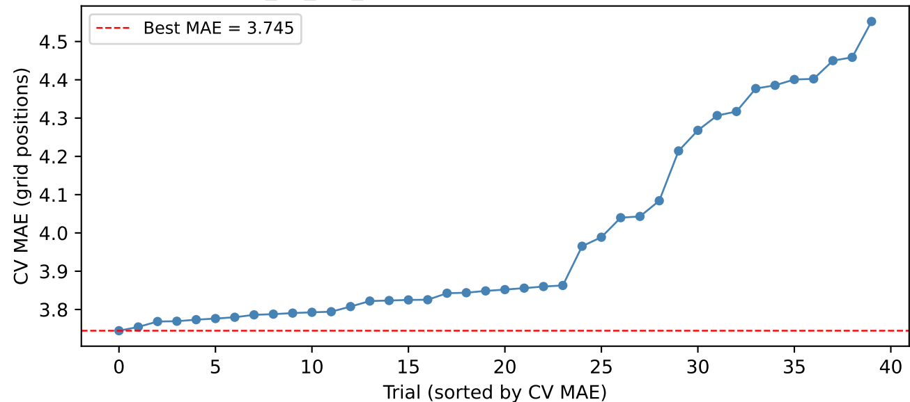
MLP_no_fp1_fp2: Hyperparameter Search Results
