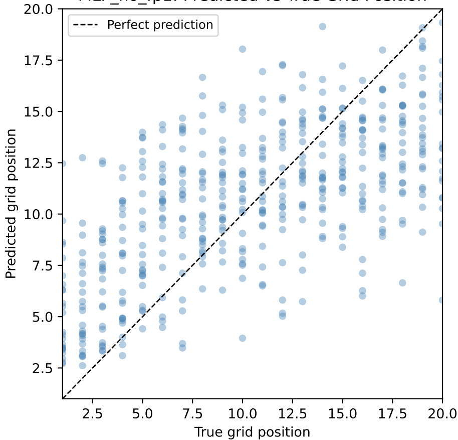
MLP_no_fp1: Predicted vs True Grid Position
