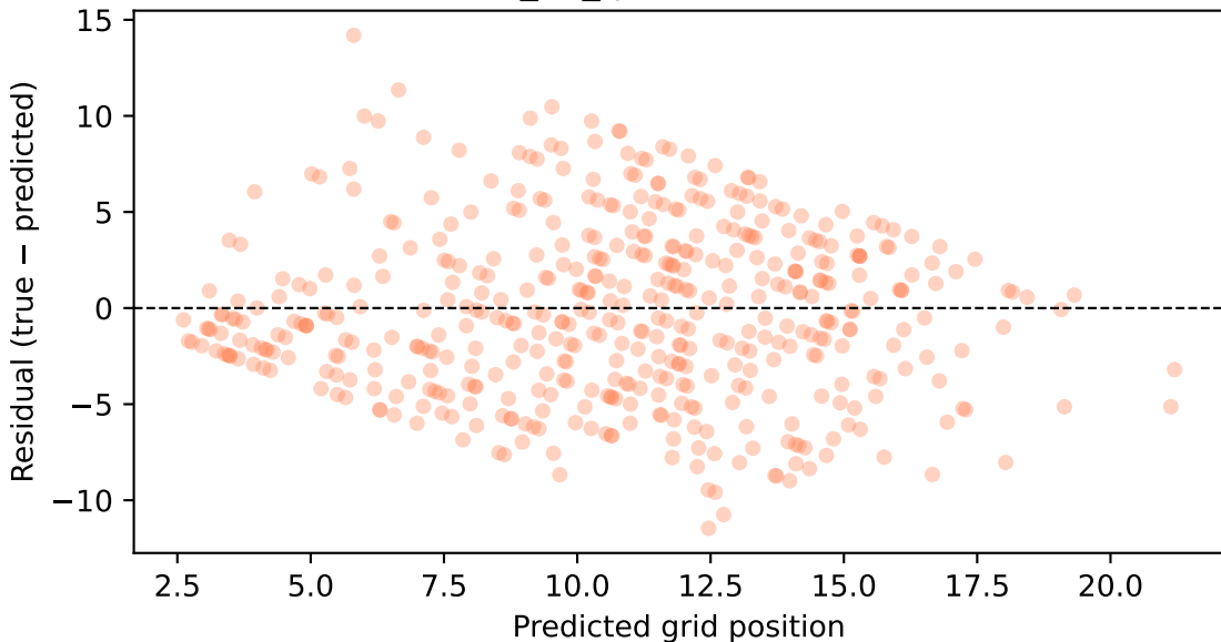
MLP_no_fp1: Residual Plot
