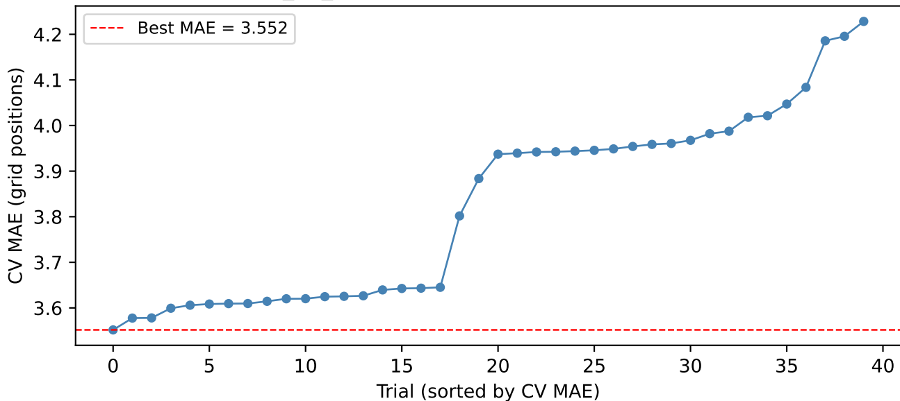
MLP_no_fp1: Hyperparameter Search Results
