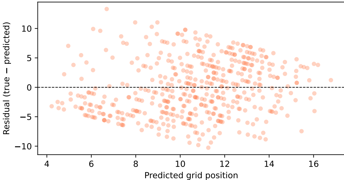
SVR_no_fp1_fp2: Residual Plot
