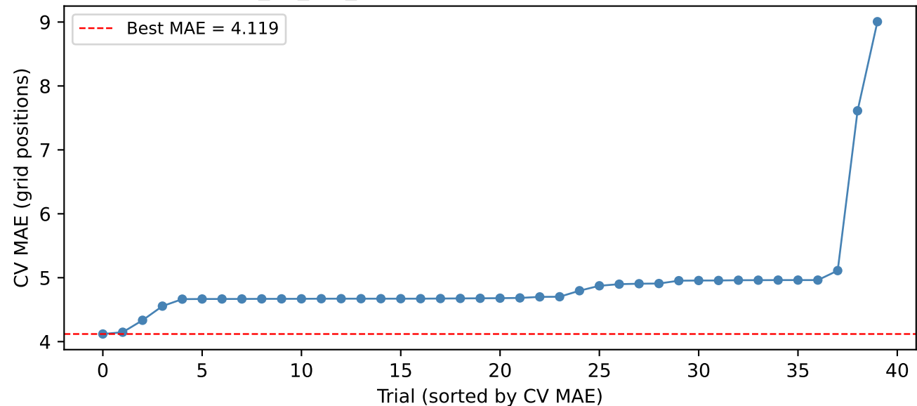
SVR_no_fp1_fp2: Hyperparameter Search Results
