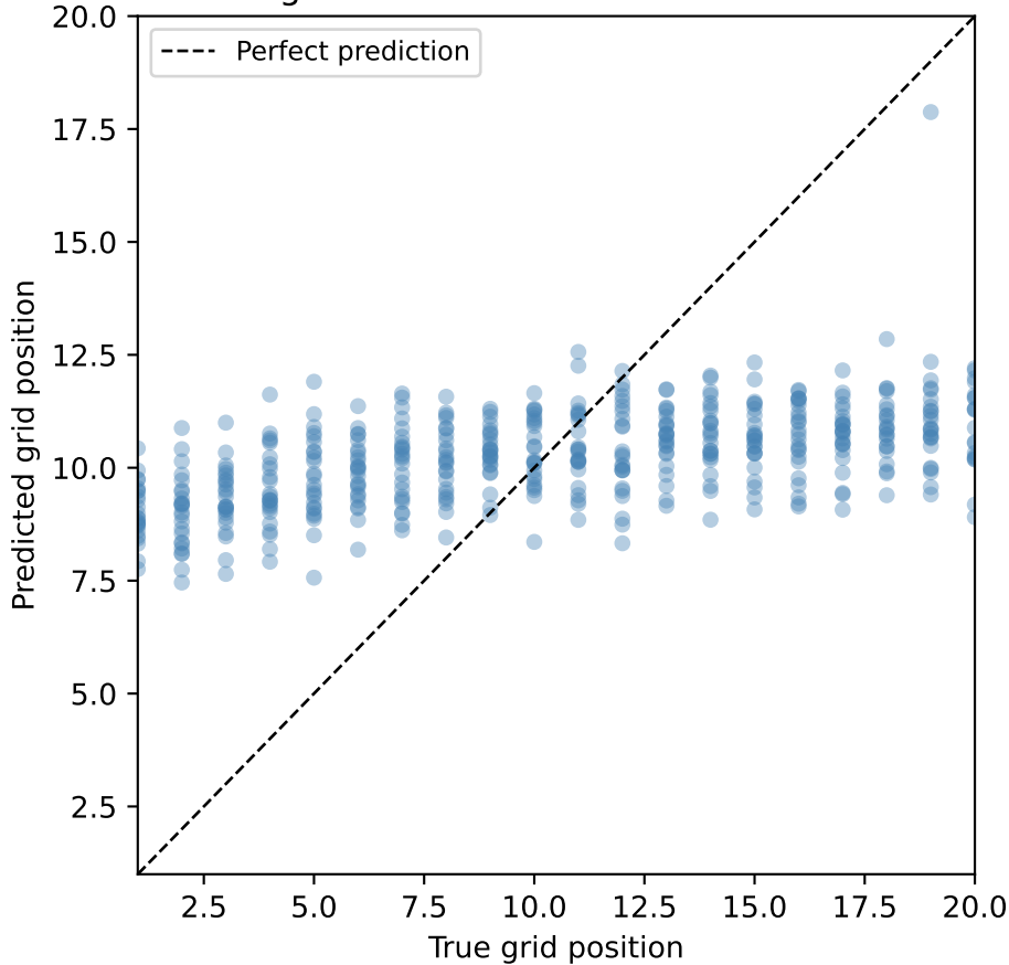
LinearRegression: Predicted vs True Grid Position
