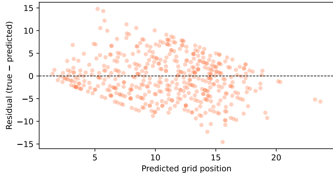
MLP: Residual Plot
