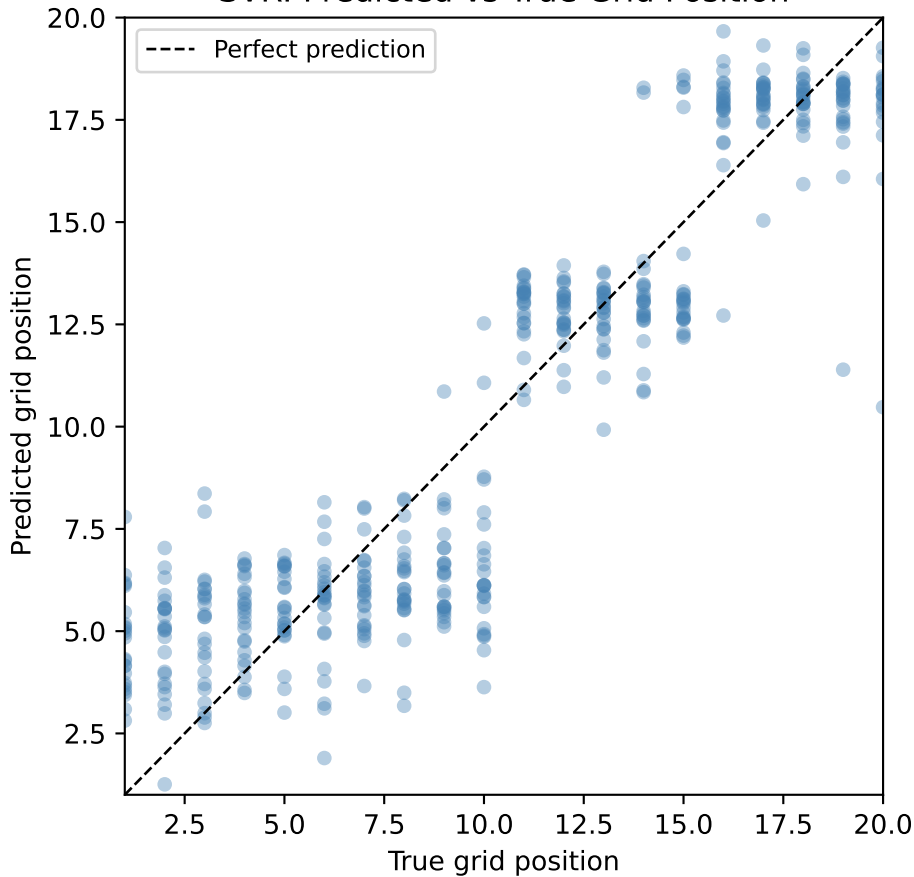
SVR: Predicted vs True Grid Position
