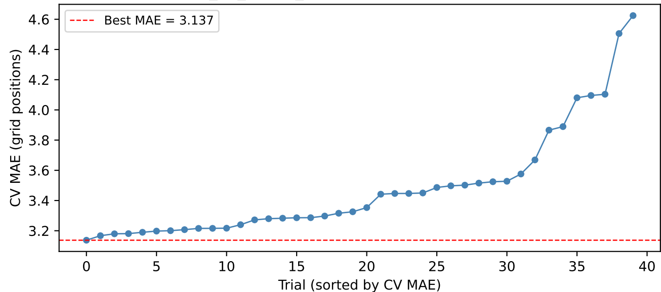
GradientBoosting_no_circuit_metadata: Hyperparameter Search Results
