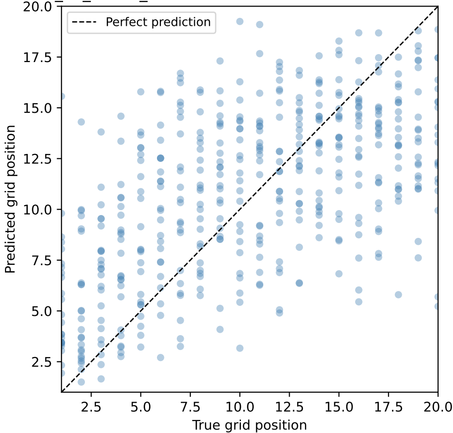
MLP_no_circuit_metadata: Predicted vs True Grid Position
