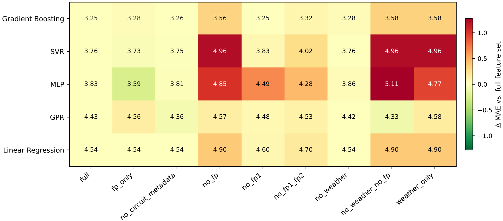
Feature ablation analysis: MAE by model and ablation (cell values = MAE; color = change from full feature set)
