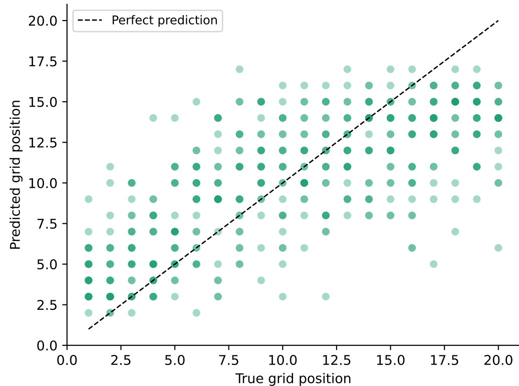
Gradient Boosting: predicted vs. true grid position
