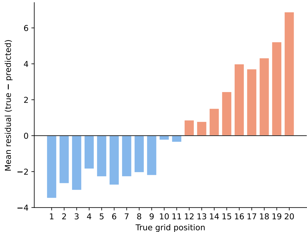
Gradient Boosting: systematic bias by grid position
