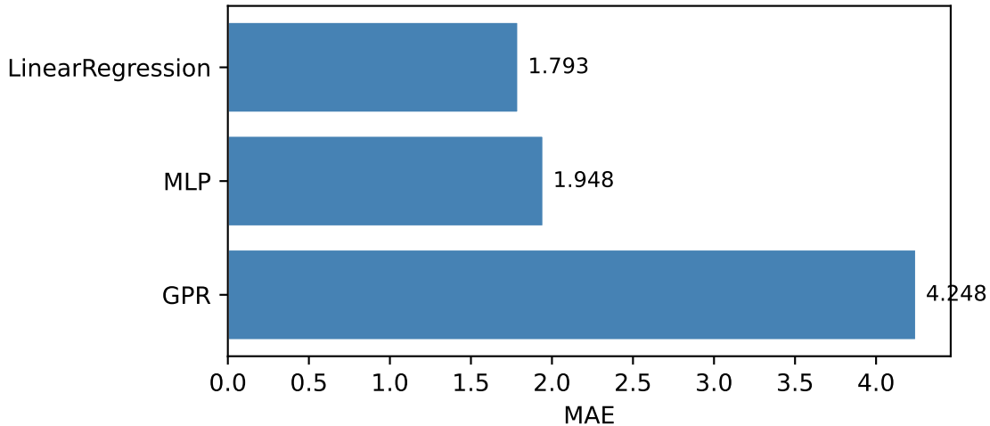
Model comparison — MAE
