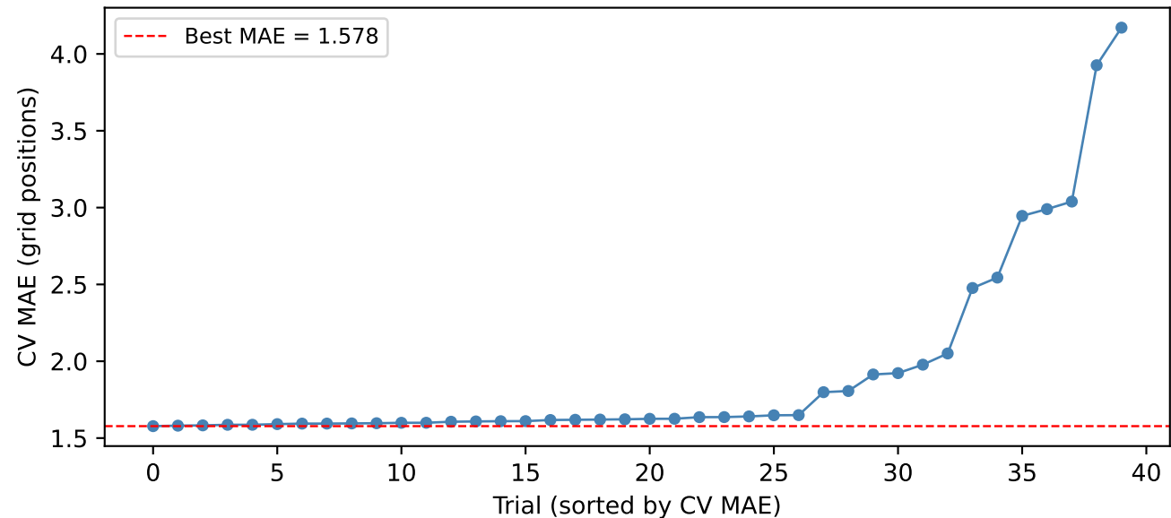
GradientBoosting: Hyperparameter Search Results
