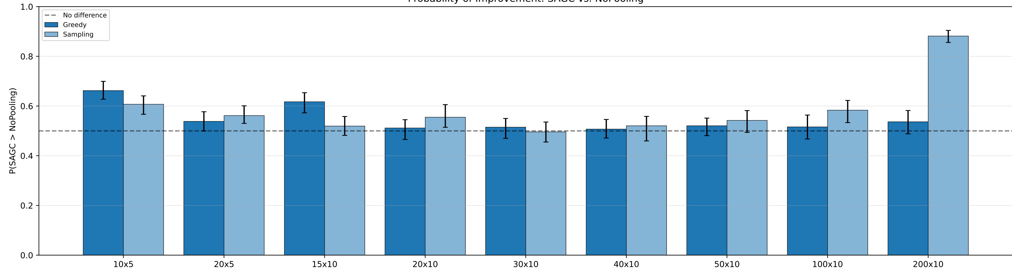
Probability of Improvement: SAGC vs. NoPooling
