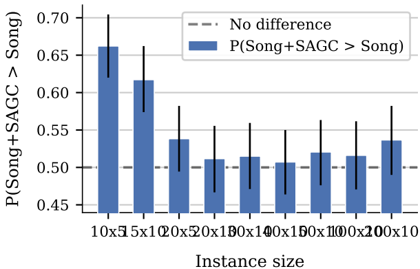
Greedy
