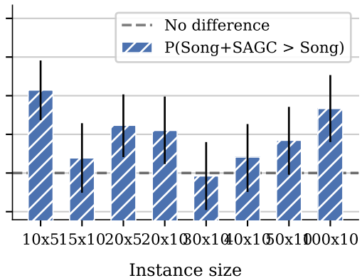
Sampling
