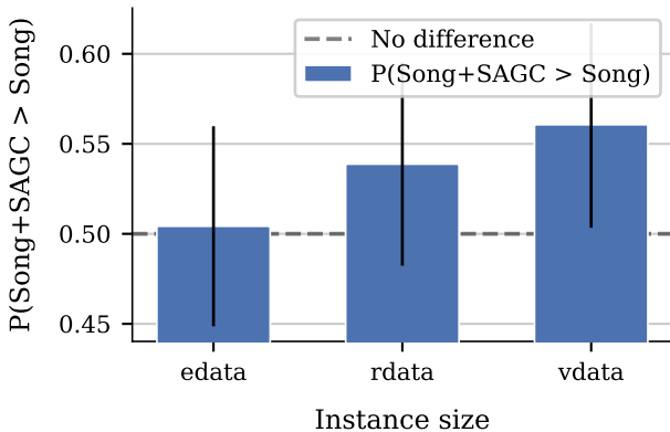
Greedy
