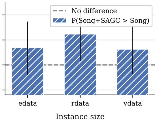
Sampling
