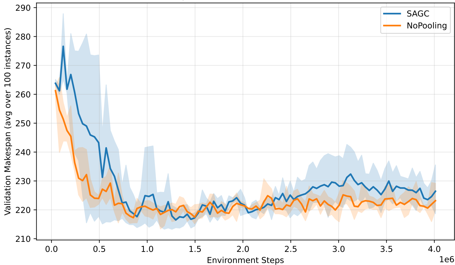
Training Curves on 20x10 Validation Set
