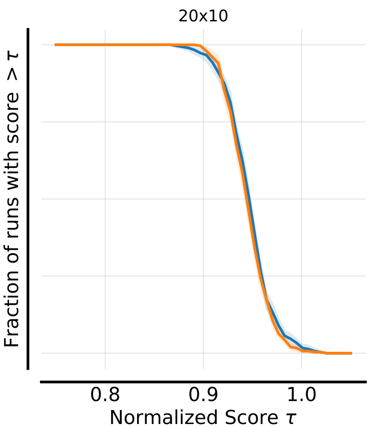
Performance Profiles with 95% Bootstrap Confidence Bands
