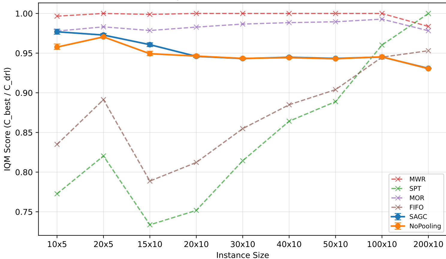
Scaling: Performance over Instance Size
